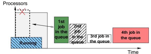
(a) Jobs 1, 2, 3 and 4 arrive in the queue and have to be scheduled
