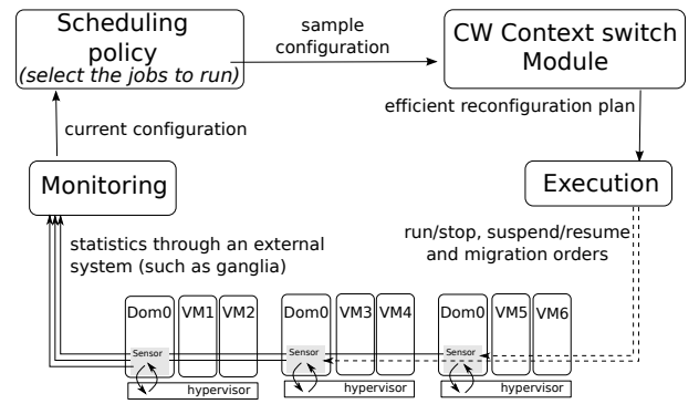
Figure 4: The control loop of Entropy
