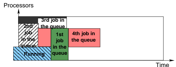
(c) EASY back filling with preemption. The job 4 is started earlier without impacting job 1. A small piece of resources is still unused (dark gray areas). Thanks to the consolidation and preemption mechanisms, it is possible to improve the whole cluster usage.
