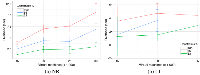
Fig. 3: Impact of the user constraints over the solution time
